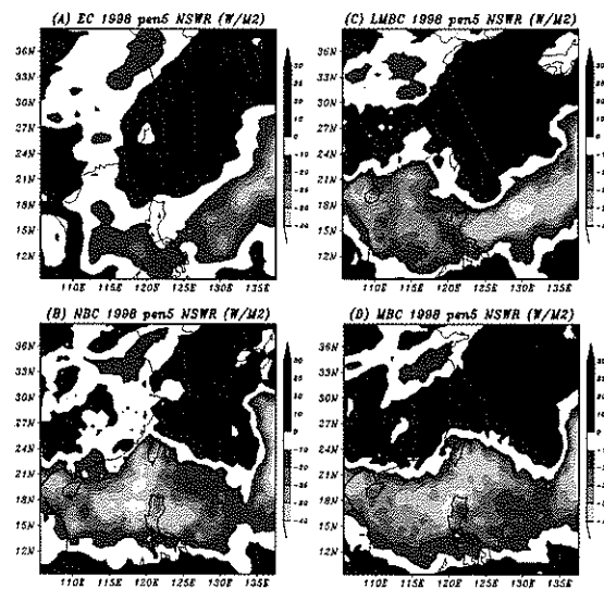
Fig. 4. Pentad mean of the observed and simulated horizontal structure of net shortwave radiation anomalies ( W/M^2 ) for (A) EC, (B) NBC run, (C) LMBC run, and (D) MBC run. The anomaly is obtained from subtracting the monthly net shortwave radiation of May 1998 from 6 hr net shortwave radiation.
