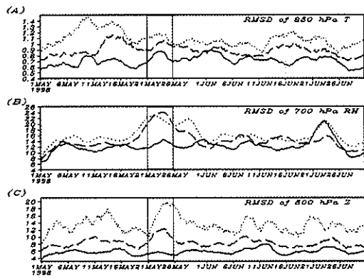
Fig. 5. Temporal evolution of RMSD for (A) 850 hpa temperature (K), (B) 700 hpa relative humidity (%), and (C) 500 hpa height (m). Each plot shows three cases: NBC (dotted), LMBC (solid), and MBC (dashed). Solid line area denotes SCS summer monsoon onset period.
