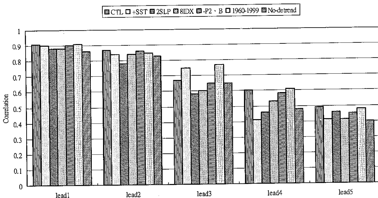
Nino3.4 Cross-validation for DJF
