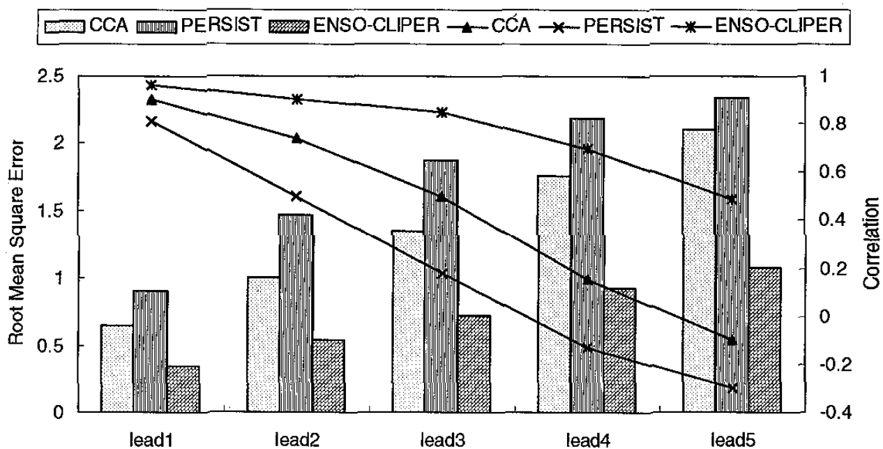
Nino3.4 Verification (1996-2000)
