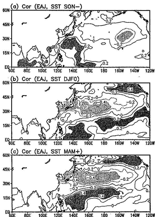
Fig. 5. Correlation between the EAJ and grid-point SST. Shown are the simultaneous pattern (b) and the patterns in which the SST leads the EAJ by one season (a) and lags the EAJ by one season (c). Values \geq 95\% confidence level are shaded.
