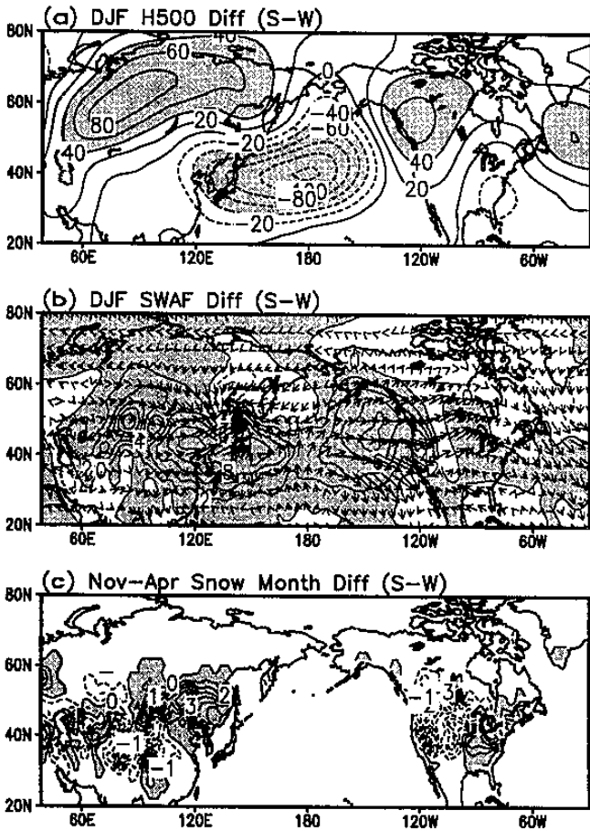
Fig.3. Differences, between strong and weak EAJs, in the number of month of H500 (a; in m), SWAF (b), and snow cover (c; in month). In (b), the vectors are for 300 mb horizontal component and the contours and shadings for 850 mb vertical component (see text for units).
