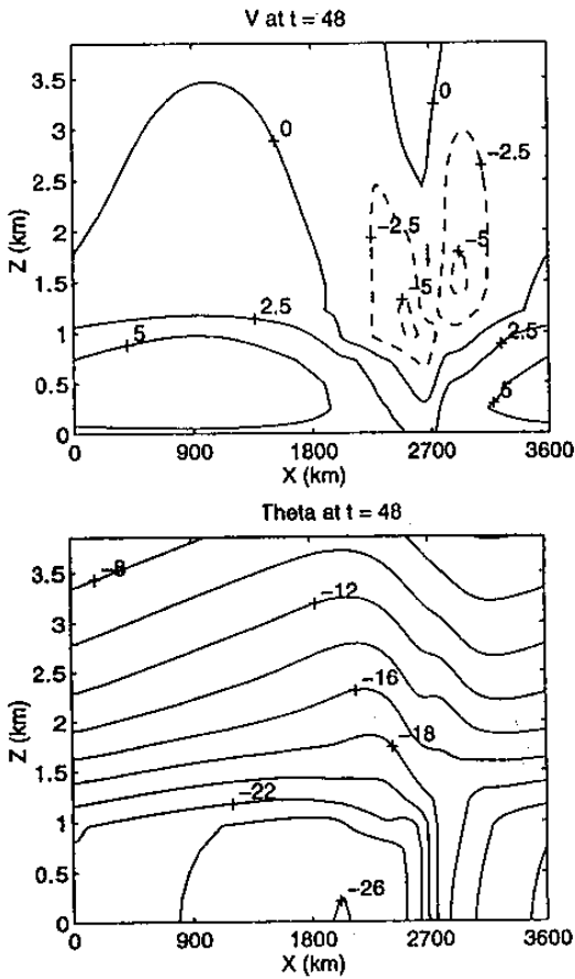
Figure 2. Same as in Fig. 1 except with PBL.
