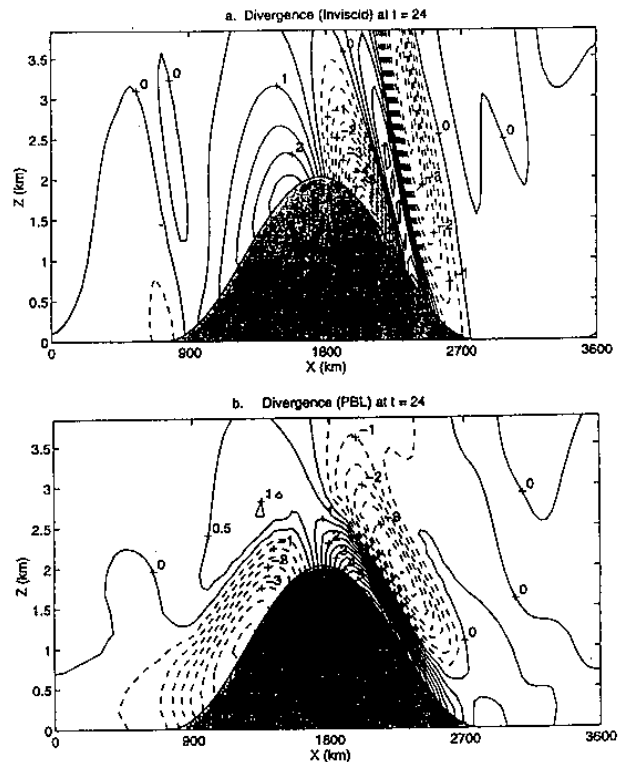
Figure 6. Divergence field at t = 24 h for; a) the inviscid mountain and b) the mountain with PBL.
