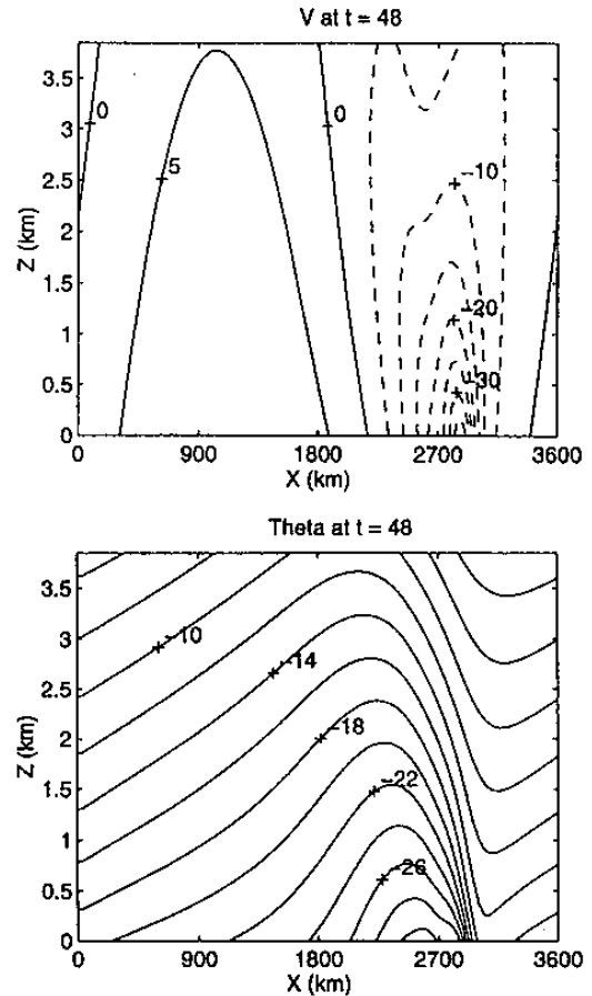
Figure 1. (a) Along-front wind component and (b) potential temperature for inviscid front at t = 48h .
